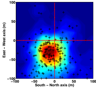
Figure 3: Difference between shower core positions obtained from radio signals and from the scintillator array. Each black cross is one EAS core position and a smoothed density map is superimposed. Instead, a systematical shift of the radio core of \sim 20 m toward the East is observed.
