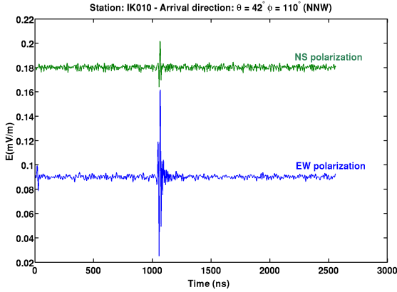
Figure 5. Wave shape for both EW and NS polarizations of the electric field filtered in the 30-80MHz band.
