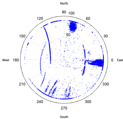
Figure 3. Arrival direction of the reconstructed events for one day of data taking. We can observe the trajectory of some planes and a large number of events near the horizon, that correspond to noise sources.
