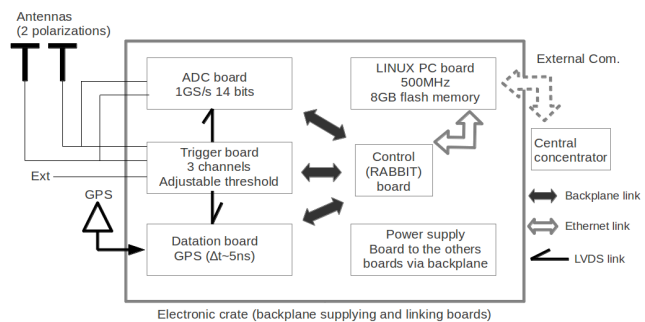
Figure 2. Schematic description of the station elements.
