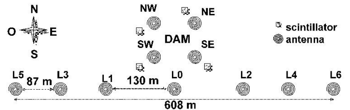
Figure 1. Layout of the CODALEMA set-up
