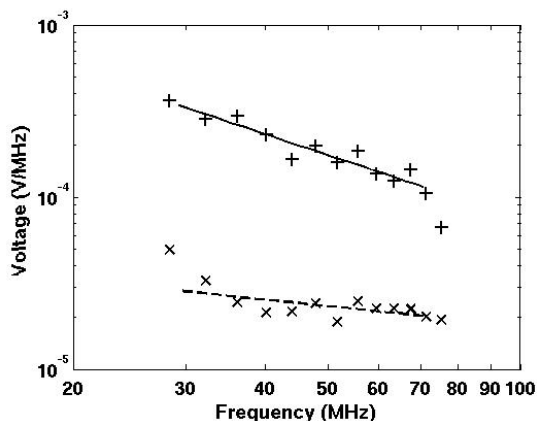
Figure 6. Voltage frequency spectra of both the signal and the background. Full and dashed lines correspond to least square fits.
