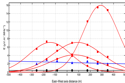
Figure 2. Profile of the maximum voltage (corrected from the cable attenuation and the amplifier gains) recorded on the antennas in the East-West direction for 4 EAS events (squares, gaussian fit: red/full line), an anthropic transient (triangles, fit: blue/dashed line) and detection thresholds (circles, fit: black/dash-dotted line).
